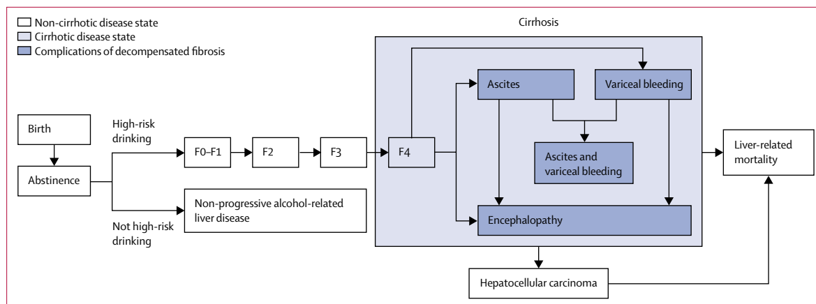
Figure 1: State-transition model of the natural history of alcohol-related liver disease
