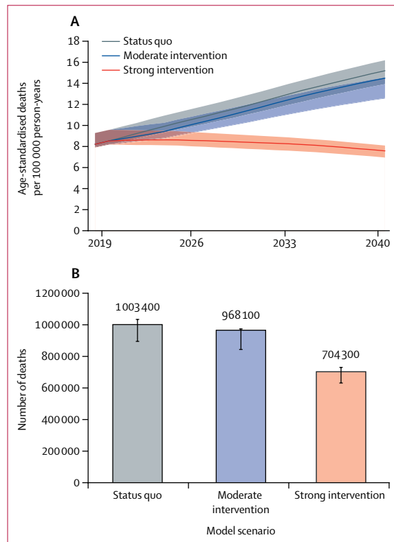
Figure 2: Model-predicted mortality due to alcohol-related liver disease in the USA, 2019–40
