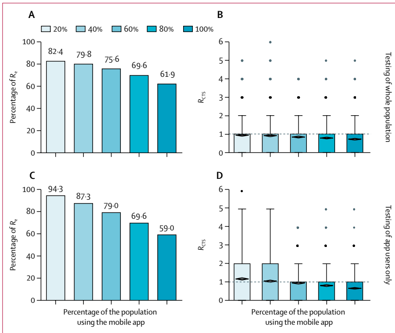
Figure 4: Impact of varying levels of mobile app use on R_{cts} In panels A and B, we assume that there is also testing (at 80% coverage) of those who do not use the mobile app, so app use only is used for tracing contacts. In panels C and D, only app users, who develop symptoms, are tested. Panels A and C show percentage reductions of R_e achieved by the mobile app contact tracing strategy; panels B and D show the impact of various contact tracing strategies on distributions of individual reproduction numbers, R_{cts} . Each boxplot shows the mean (diamond), where the height of the diamond indicates the CI of the mean) IQR, and upper fence (75% quartile + 1.5 × IQR) of the distribution. The dots are outliers, where darker dots contain more datapoints than lighter dots. All datapoints are integers. R_e =effective reproduction number. R_{cts} =effective reproduction number with contact tracing.
