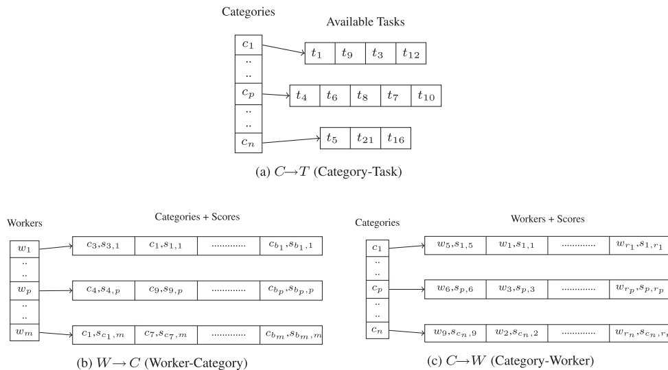
Figure 1 Data structures.
