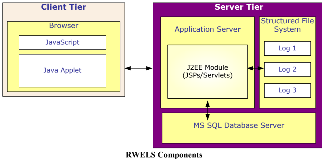
Fig. 5. The client and server side components in RWELS.
