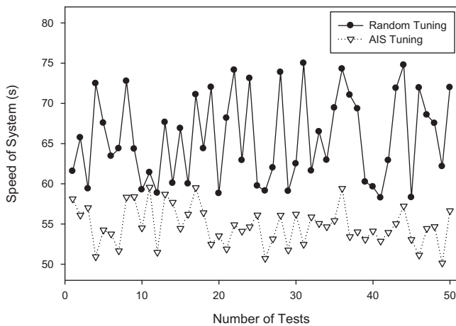
Figure 14 Speed test using optimum dispensing parameters for medium A.
