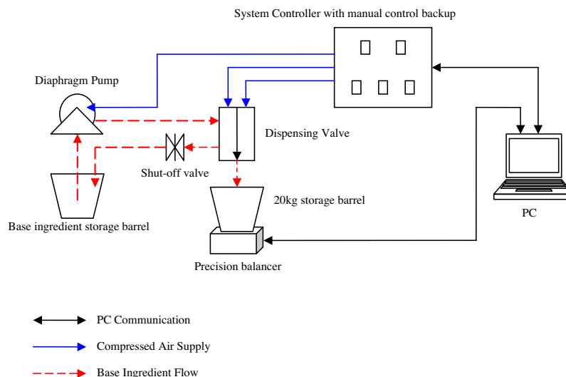
Figure 6 Gravimetric dispensing system setup.
