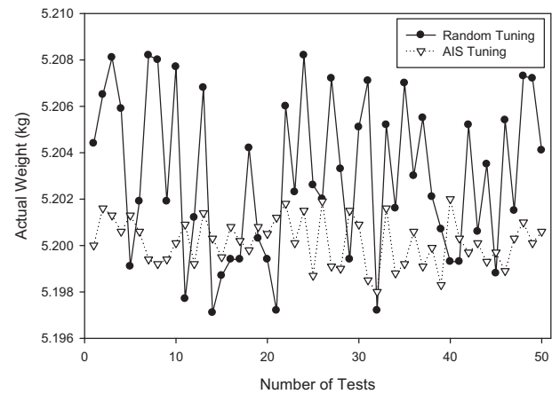
Figure 11 Accuracy test using optimum dispensing parameters for medium A.
