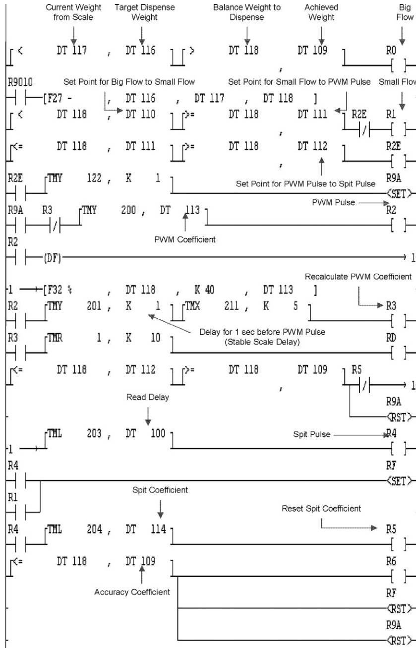
Figure 5 Control mechanism of PLC.
