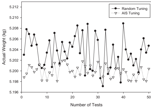
Figure 12 Accuracy test using optimum dispensing parameters for medium B.
