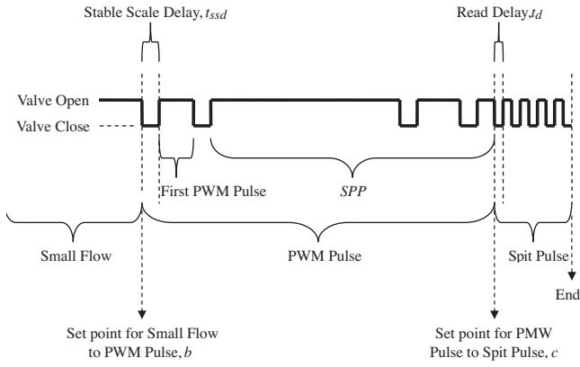
Figure 3 Timing diagram for PWM pulse technique.
