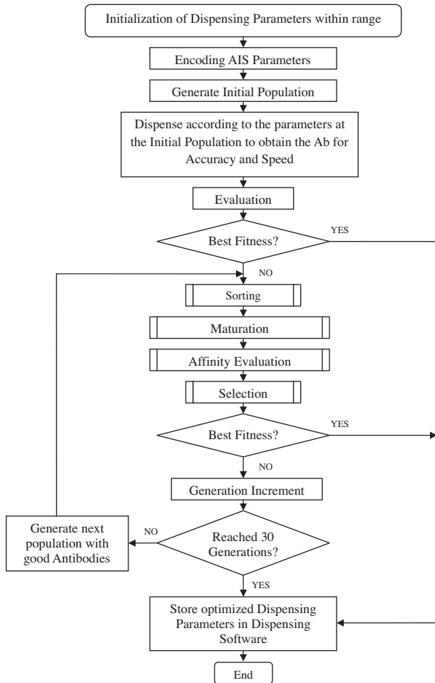
Figure 10 Flow chart of the AIS dispensing parameter fine tuning program.
