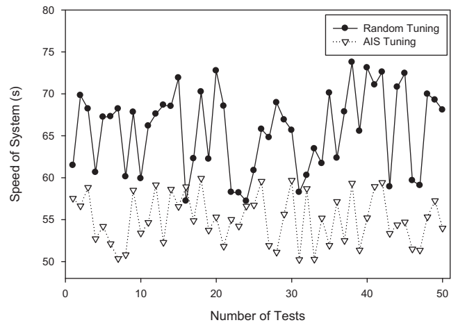
Figure 15 Speed test using optimum dispensing parameters for medium B.
