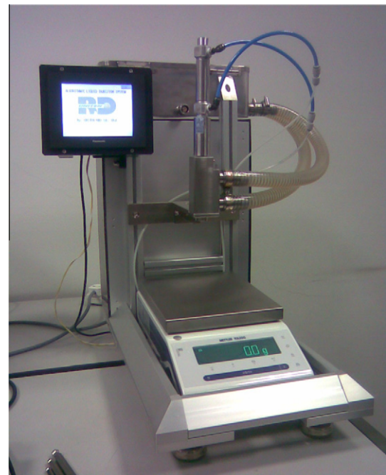
Figure 7 Developed fluid dispensing system.
