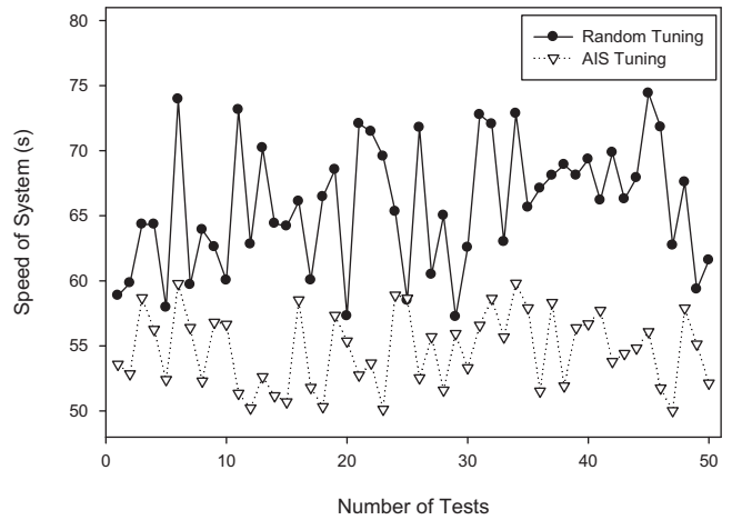
Figure 16 Speed test using optimum dispensing parameters for medium C.
