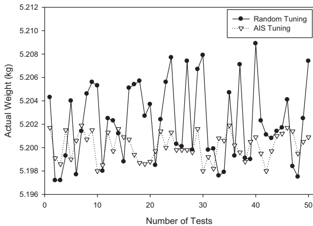
Figure 13 Accuracy test using optimum dispensing parameters for medium C.
