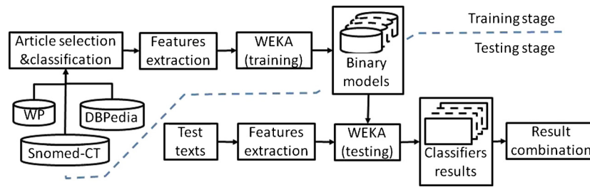
Fig. 1. Training and testing pipelines.
