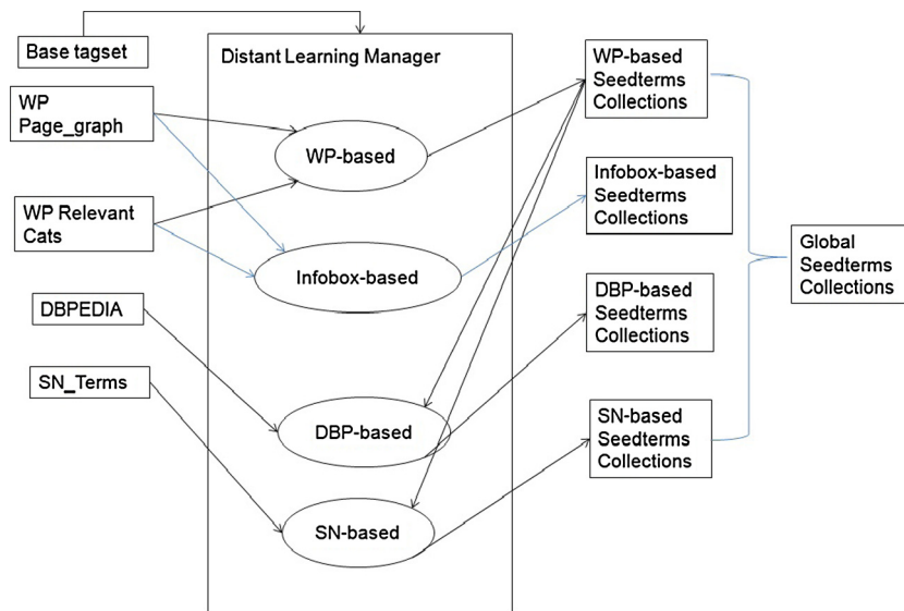
Fig. 3. Distant learning manager.
