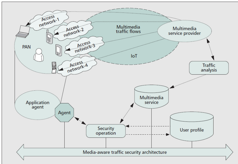
Figure 11 MTSA architecture.
